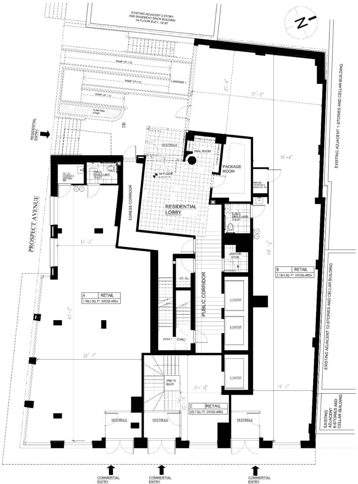
1st FLOOR PLAN
